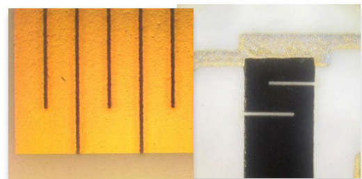
Serpentine trims in thin and thick films.
